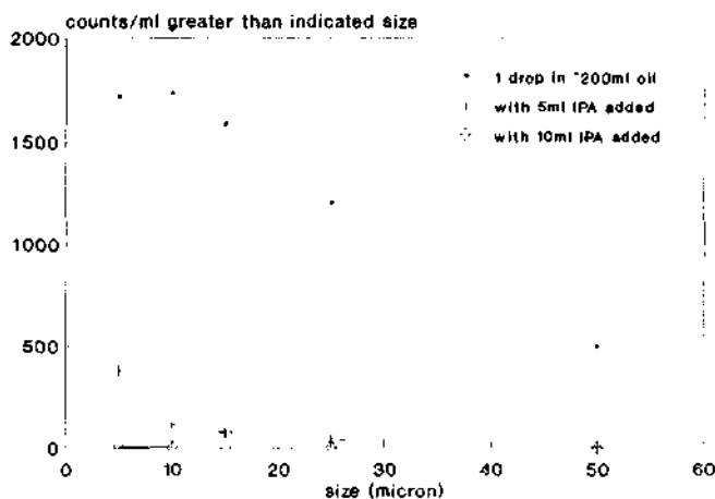
Fig 2 False counts obtained in a bottle of clean Flush Stand oil containing one drop of water and their reduction by treatment with isopropyl alcohol
