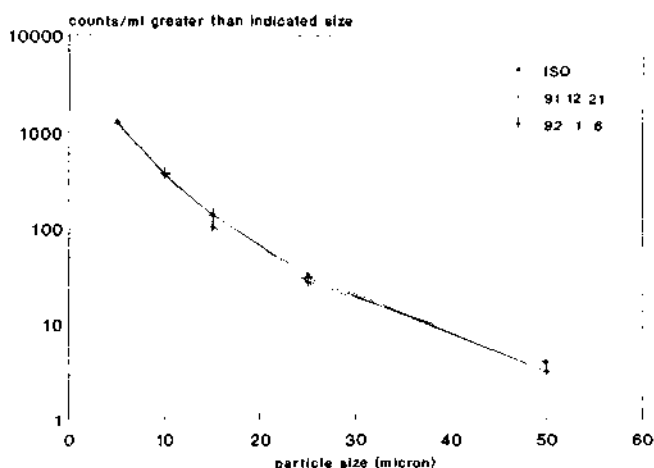
Fig 1 Particle size distribution in fluid containing 2.5 mg/l ACFTD measured on different dates and the distribution according to ISO code 4402-1977(E)
