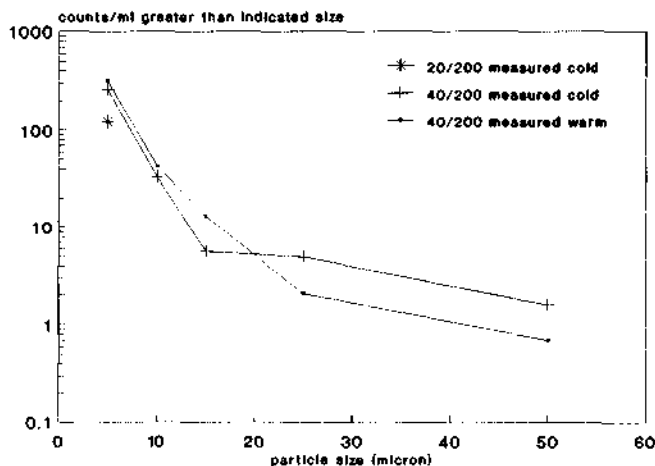
Fig 3 Particle size distribution in 200 ml fluid containing 20 ml or 40 ml centrifuged oil as measured cold or warm
