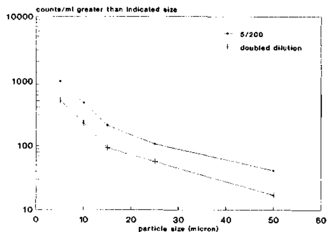
Fig 4 Particle size distribution in 200 ml fluid containing 5 ml dosed oil and at double this dilution
